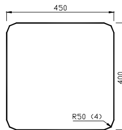
Minimum external dimensions at the section B-B
